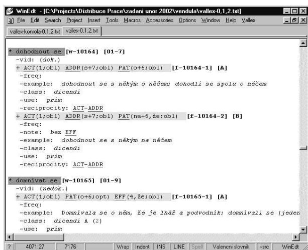
Figure 7: WinEdt screenshot.
