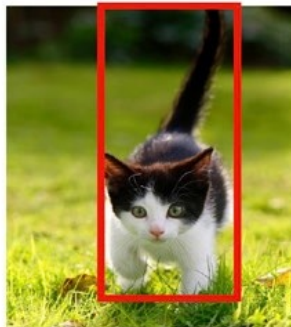
Classification + localization
