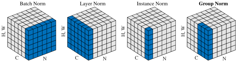
Figure 2 of "Group Normalization", https://arxiv.org/abs/1803.08494
