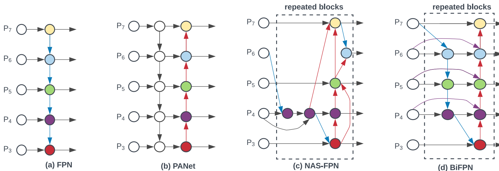
Figure 2 of "EfficientDet: Scalable and Efficient Object Detection", https://arxiv.org/abs/1911.09070
