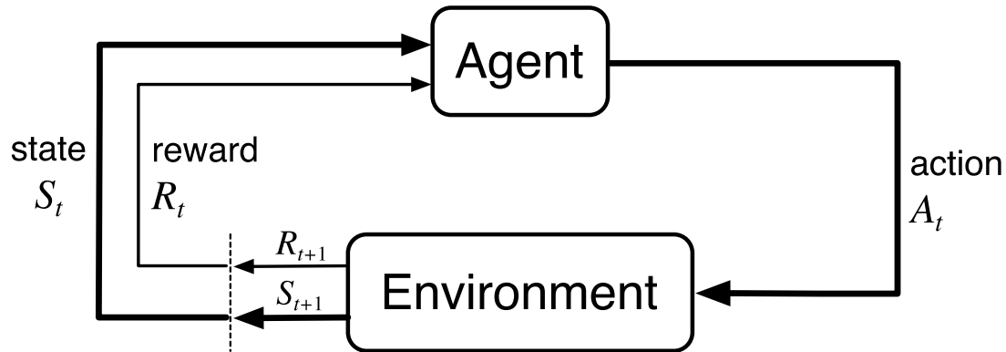
Figure 3.1 of "Reinforcement Learning: An Introduction", http://www.incompleteideas.net/book/the-book-2nd.html
