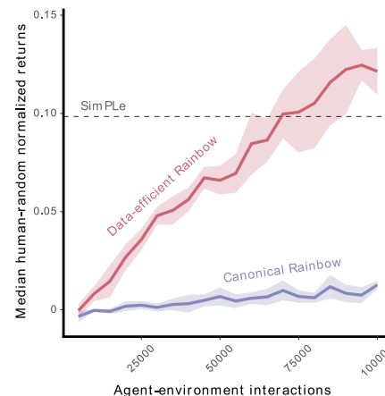
Figure 3 of "When to use parametric models in reinforcement learning?" by Hado van Hasselt et al.
