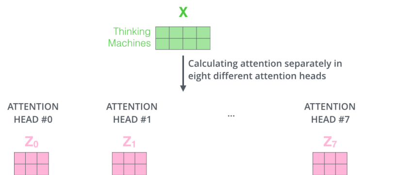
http://jalammr.github.io/images/t/transformer_attention_heads_z.png
