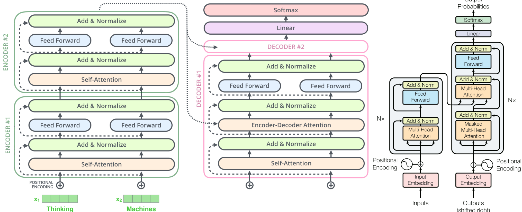
http://jalammar.github.io/images/t/transformer_residual_layer_norm_3.png
