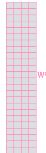
http://jalammr.github.io/images/t/transformer_attention_heads_weight_matrix_o.png
