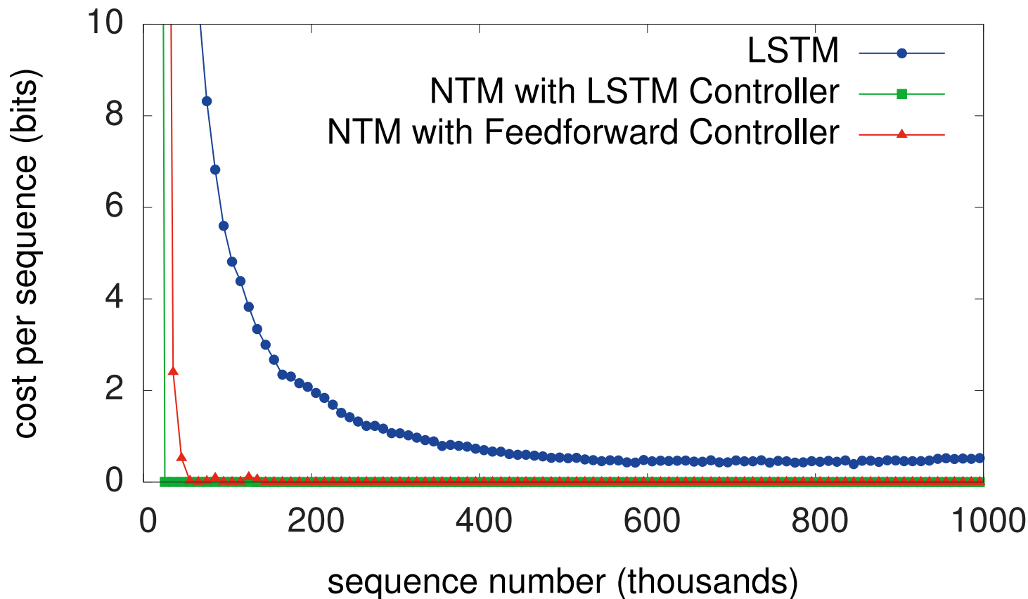
Figure 3 of paper "Neural Turing Machines", https://arxiv.org/abs/1410.5401 .
