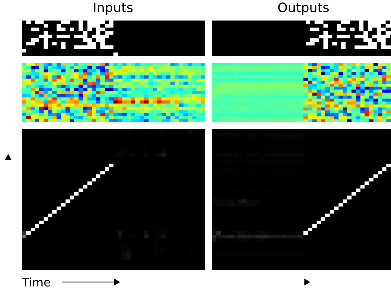
Figure 6 of paper "Neural Turing Machines", https://arxiv.org/abs/1410.5401 .
