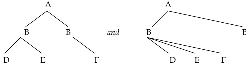
Figure 3.9: Different evaluations
