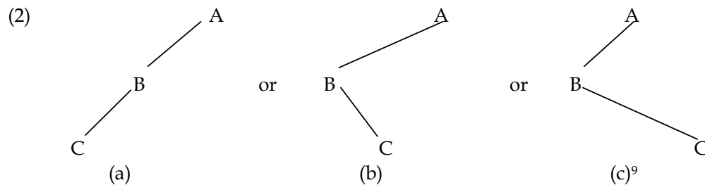
Figure 1.9 (2): A(B(C))
