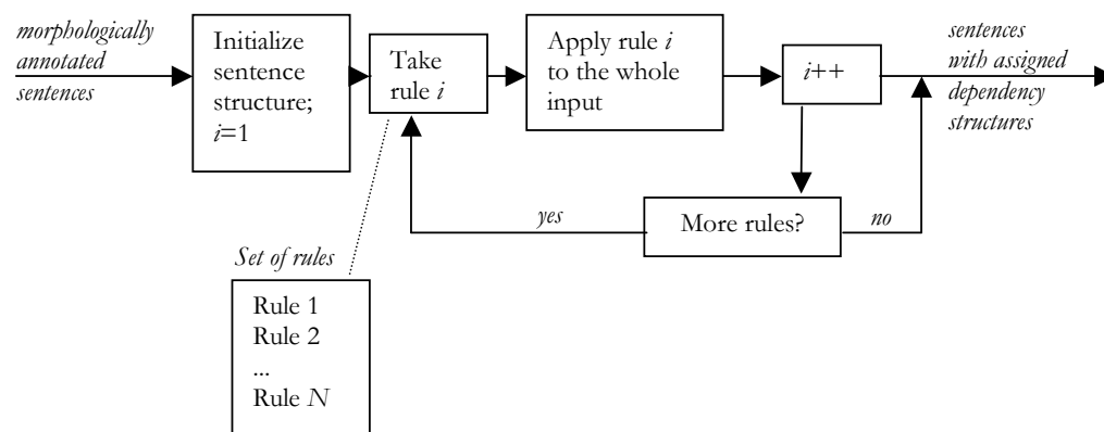
Figure 1.1: RBA - Application
