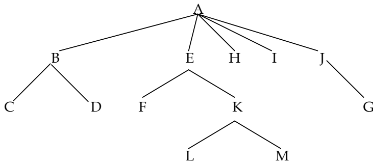
Figure 3.6: Application of SWAP COMMA BETWEEN G K
