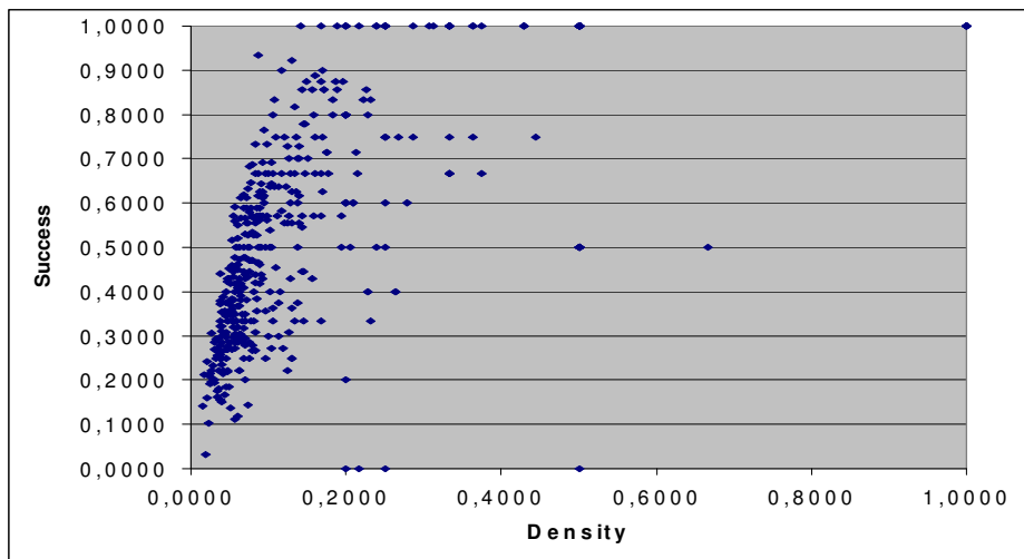
Figure 5.2: Dependency accuracy vs. sentence graph density
