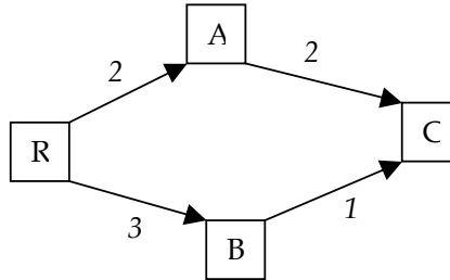
Figure 4.1: Prim's algorithm for oriented MST
