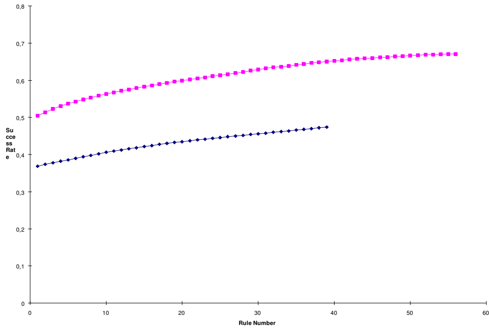
Figure 3.2: RBA learning curves
