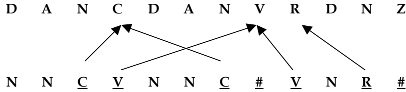
Figure 8.1: Alignment without a need of disambiguation
