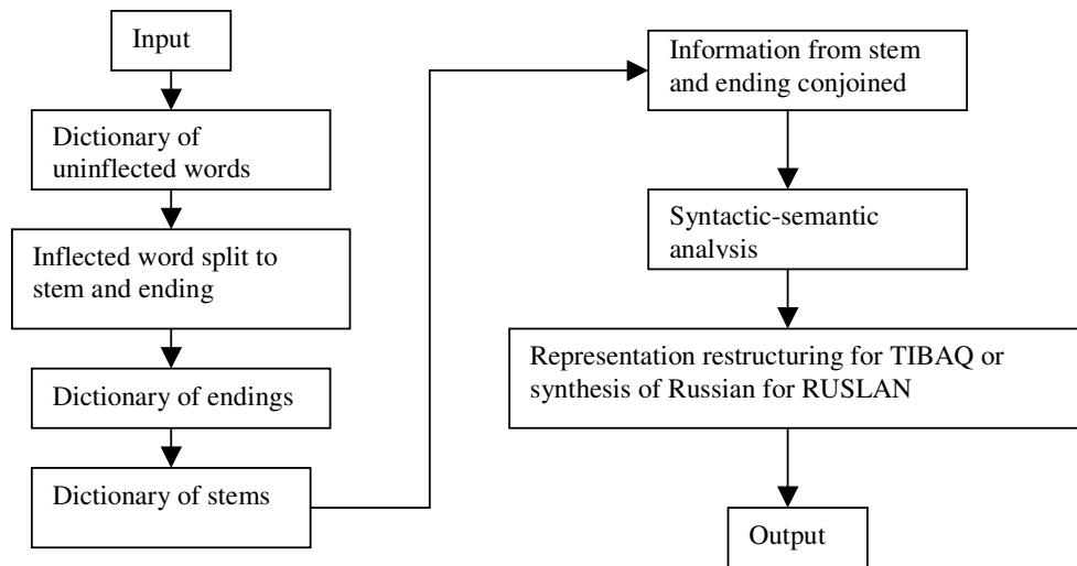
Figure 1.12: Early structure for processing (parsing) of Czech
