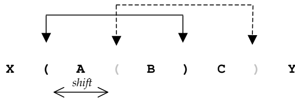
Figure 3.3: RBA for constituents
