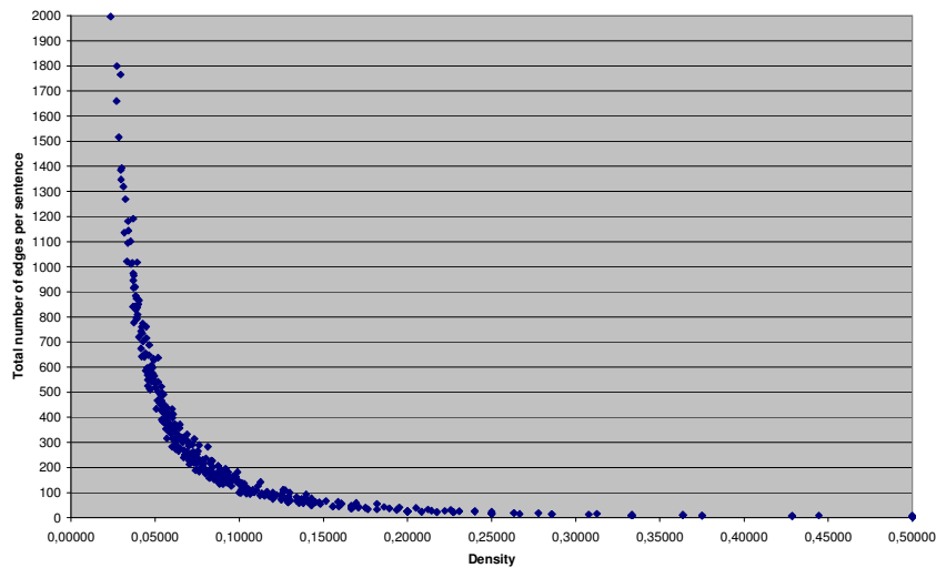
Figure 5.3: Distribution of edges in sentence graphs
