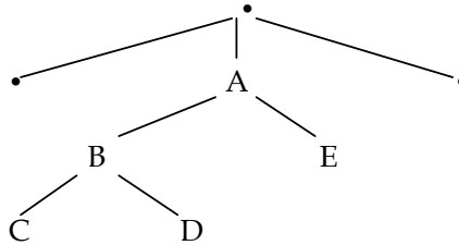
Figure 1.4: Subtree A(B(C,D),E)
