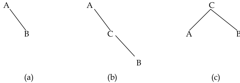
Figure 3.10: Path evaluation
