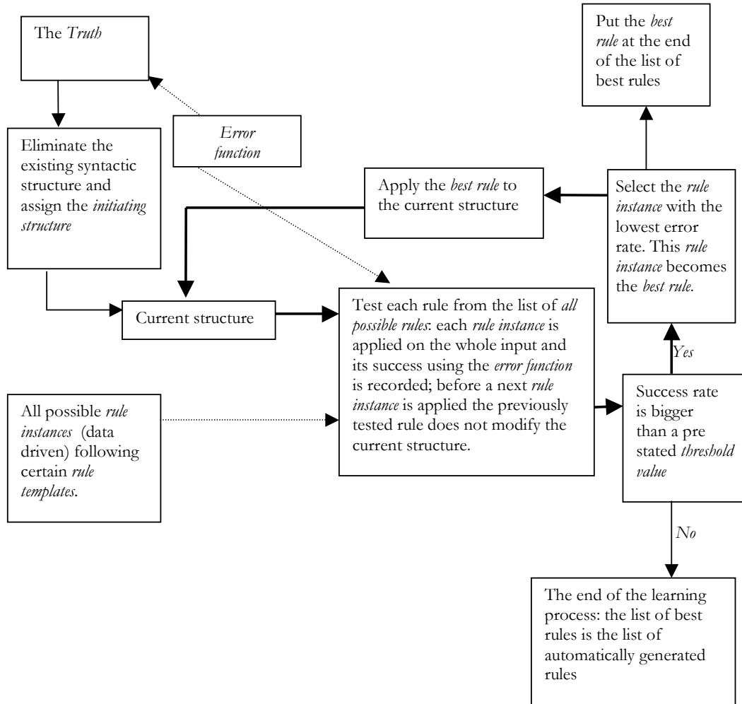
Figure 1.2: RBA - Learning
