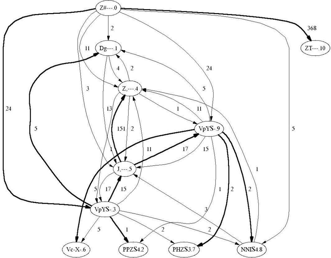
Figure 5.1: An example of a sentence graph
