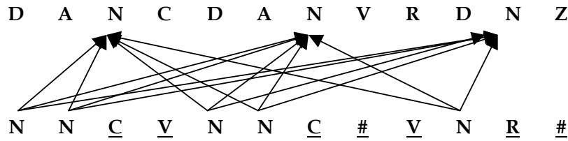
Figure 8.2: Alignment with a need of disambiguation
