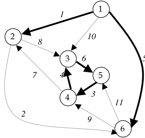
Figure 4.2: MST graph example
