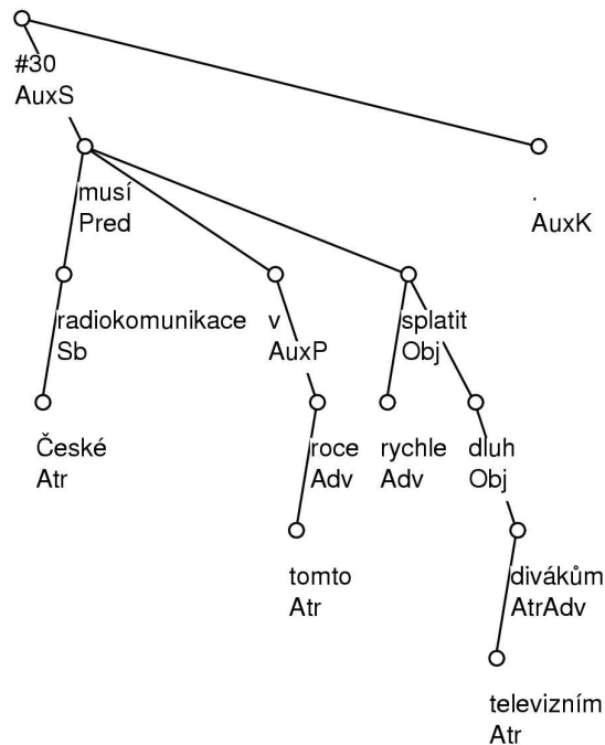
Figure 1.10: An example of an analytical tree
