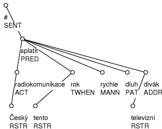
Figure 1.11: An example of a tectogrammatical tree
