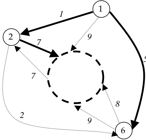
Figure 4.3: MST pseudo-vertex
