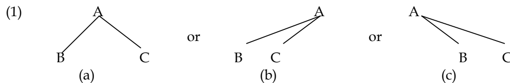
Figure 1.9 (1): A(B, C)
