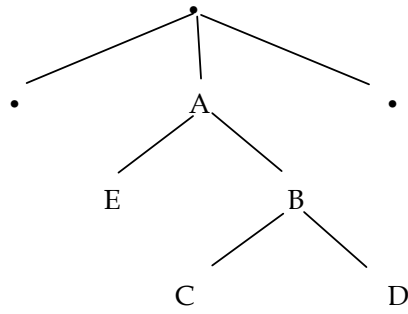
Figure 1.6: Result from SWAP COMMA BETWEEN B E
