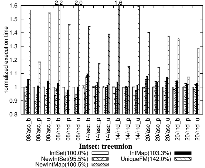
Figure 13. Benchmark of improved intsets operations II
