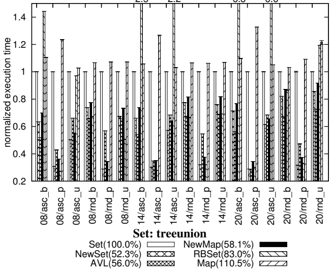
Figure 11. Benchmark of improved sets operations II
