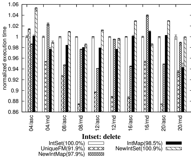
Figure 12. Benchmark of improved intsets operations I
