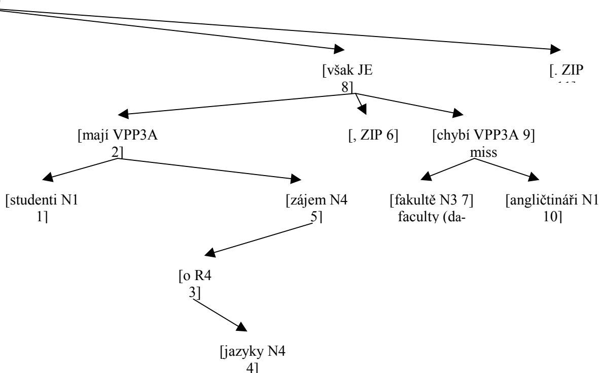
Figure 1 Example input to the algorithm from the Prague Dependency Treebank. Czech: Studenti mají o jazyky zájem, fakultě však chybí angličtináři. English: The students are interested in languages but the faculty is missing teachers of English.
