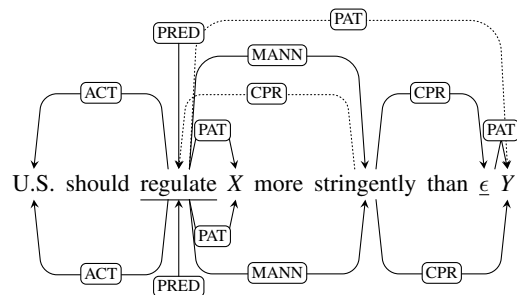
Figure 1: PCEDT asserts two copies of the token regulate (shown here as ‘regulate’ and ‘ε’ and underlined). Projecting t-nodes onto the original tokens, required by the SDP data format, means that the ε node will be merged with regulate . The edges going to and from ε will now lead to and from regulate (see the dotted arcs), which results in a cycle. To get rid of the cycle, we skip ε and connect directly its children, as shown in the final SDP graph below the sentence.
